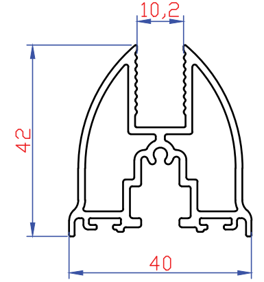
2131 935 gr/mt Gold Baza 10 mm
