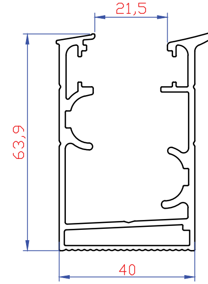
8708 R1 1354 gr/mt Gold Kasa Yeni
