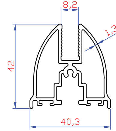
2398 875 gr/mt Gold Baza 8 mm
